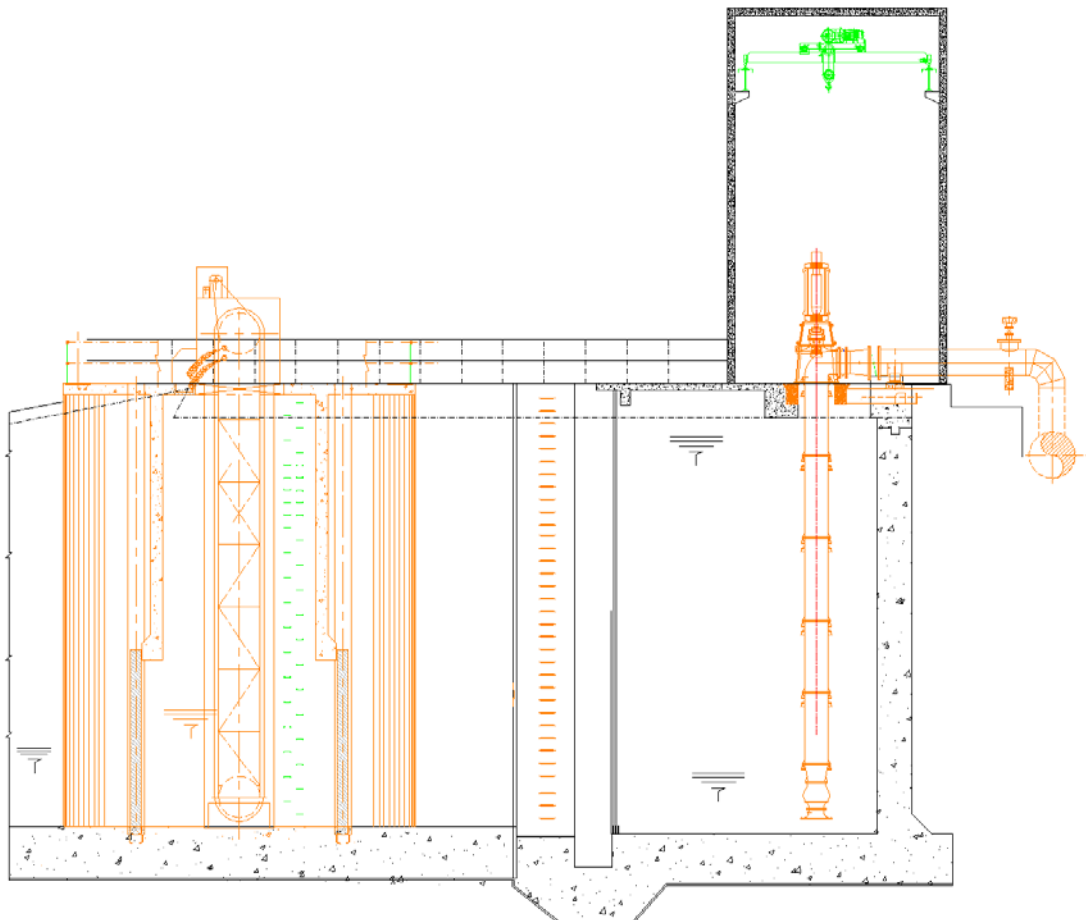
SEA WATER INTAKE SYSTEM AND PUMP HOUSE
